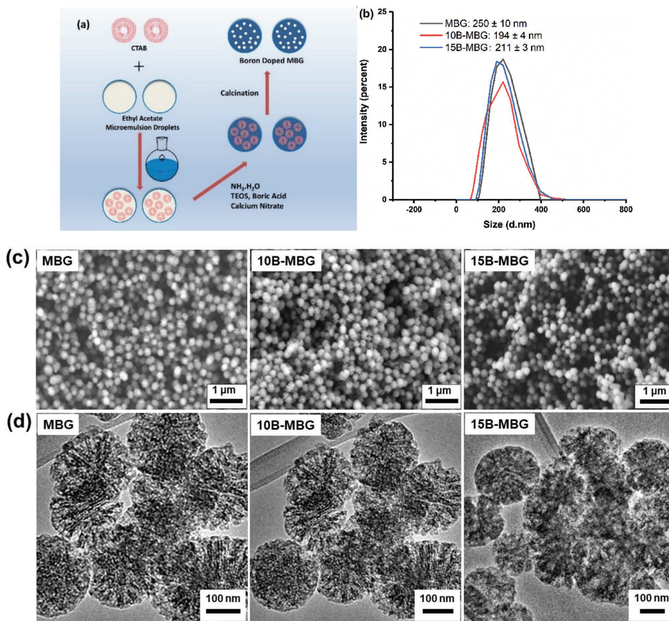
Figure 1. a) Schematic illustration of the sol–gel synthesis process; b) particle size distribution obtained by DLS measurements, c) SEM images and d) TEM images of MBG, 10B-MBG, and 15B-MBG.
